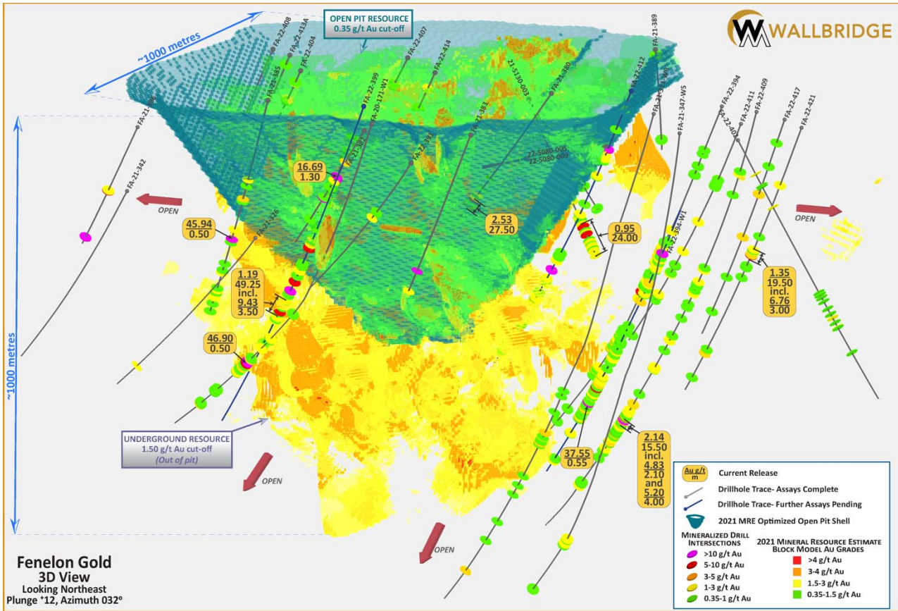
Figure 2. Fenelon, 3D View Looking Northeast
